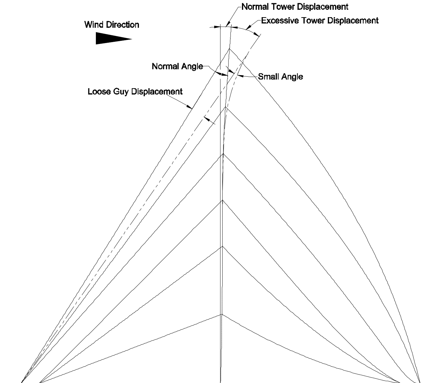
Picture 4-15: Snap-through diagram
