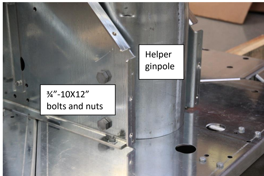
Picture 3-62: Helper ginpole attached with bolts/nuts
