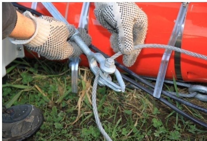
Picture 3-52: Attach jumper strut cable to turnbuckle
