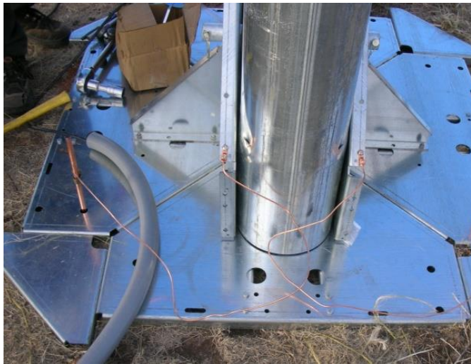
Picture 3-13: Tower Grounding
