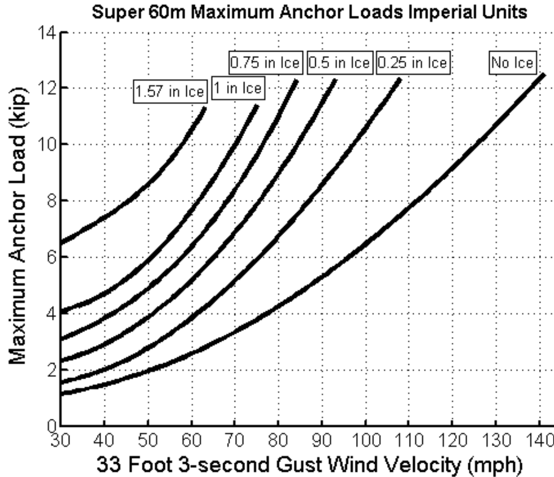
Picture A-6: Super 60 m XHD Maximum Anchor Loads Imperial Units
