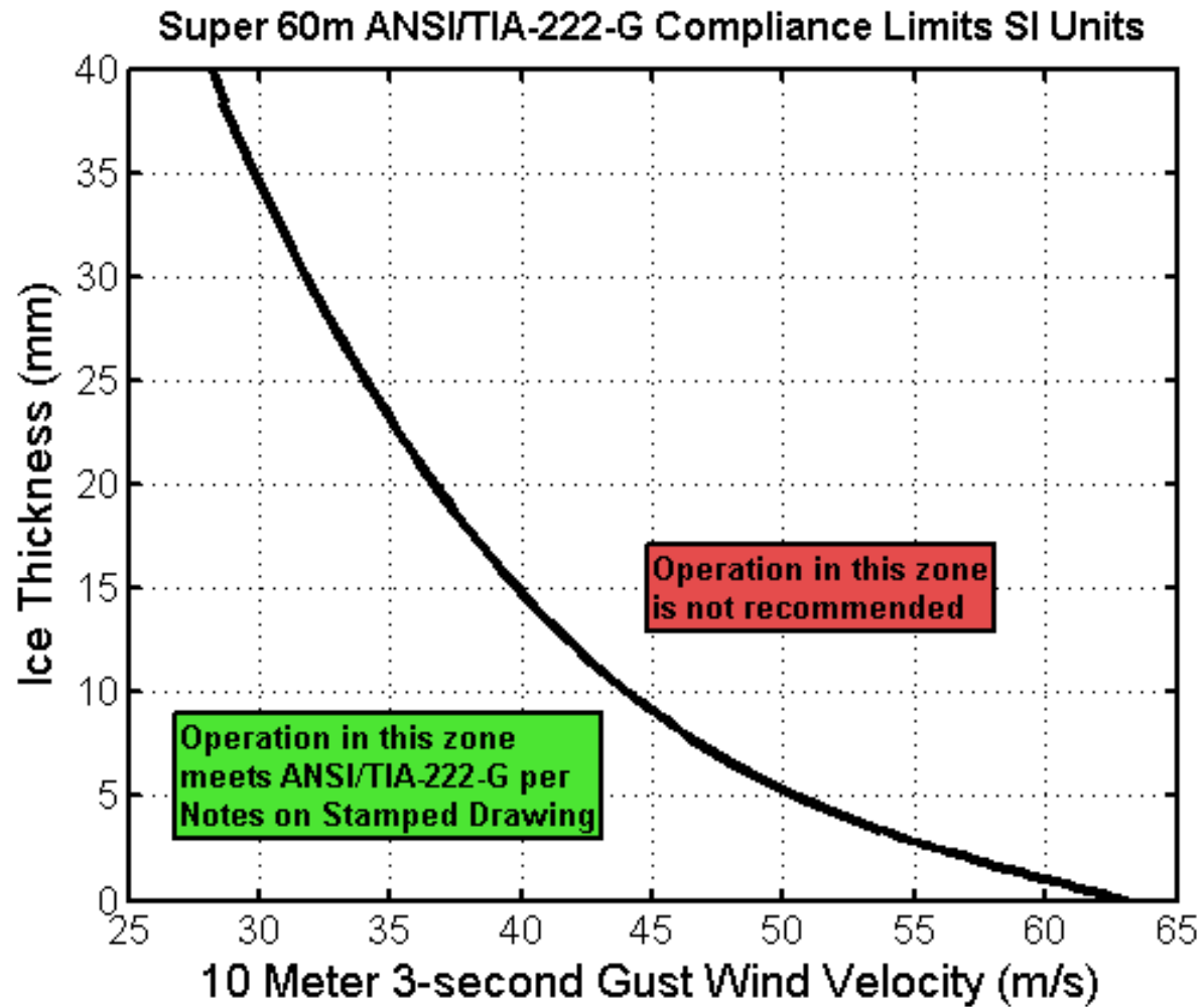
Picture A-5: Super 60 m XHD TallTower ANSI/TIA-222-G Compliance Limits SI Units
