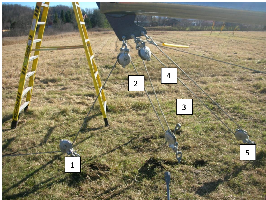
Picture 3-71: Proper winch cable reeving through block pulleys
