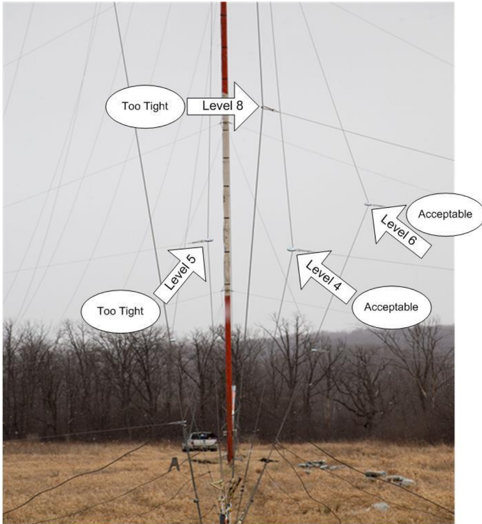
Picture E-10: View along tower showing acceptable and unacceptable back guywires/leader line tensions (Picture shows 80m tower with 8 back guy wires. Super 60 utilizes 6 back guy wires).
