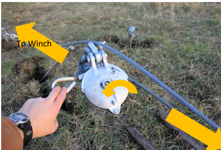
Picture 3-74: Reeving through pulley #3
