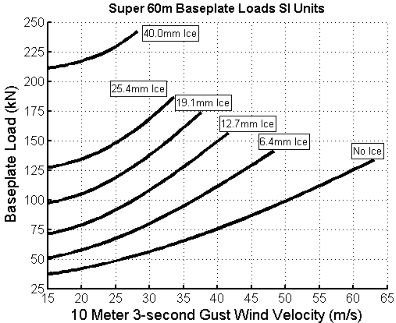
Picture A-9: Super 60m Maximum Baseplate Loads SI Units
