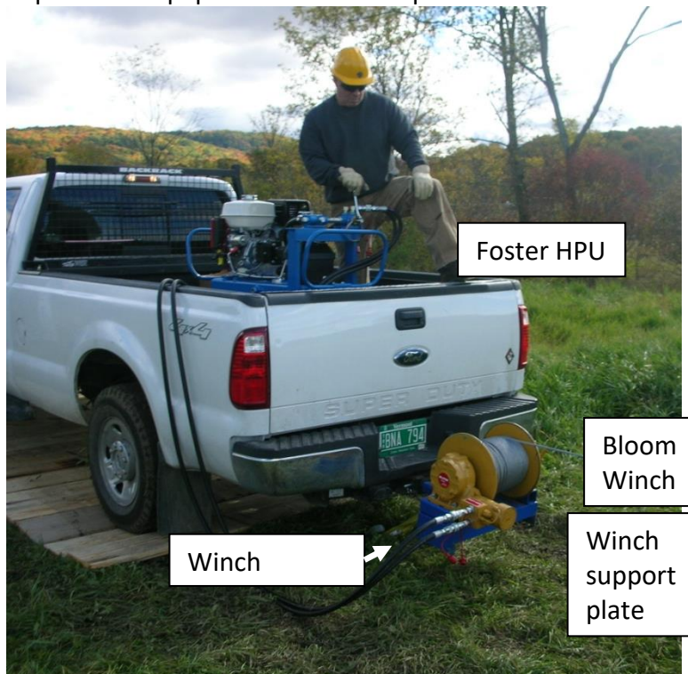
Picture 3-67: Winch set-up
