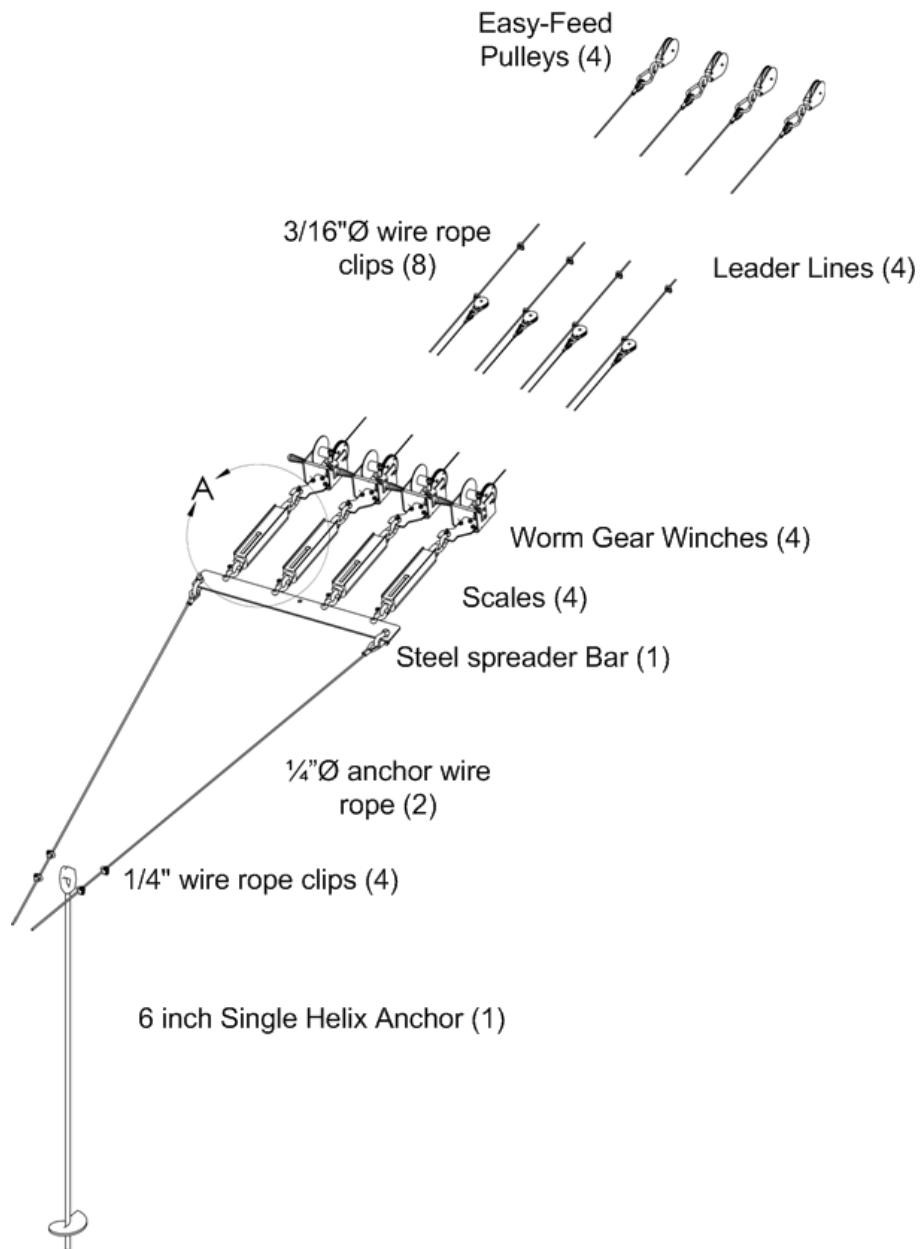
Picture E-1: Back guywire tensioner system
