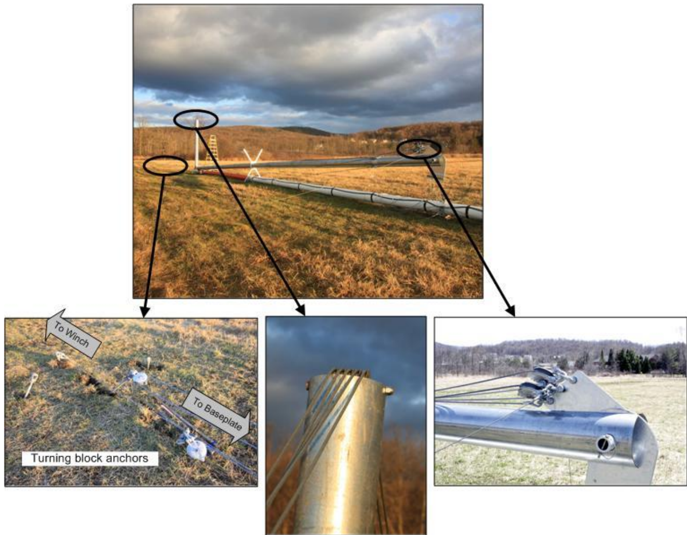
Picture 3-70: Correct reeving of the winch cable
