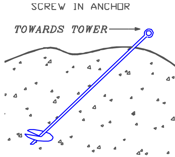
Picture B-1: Installing Screw-in Anchors
