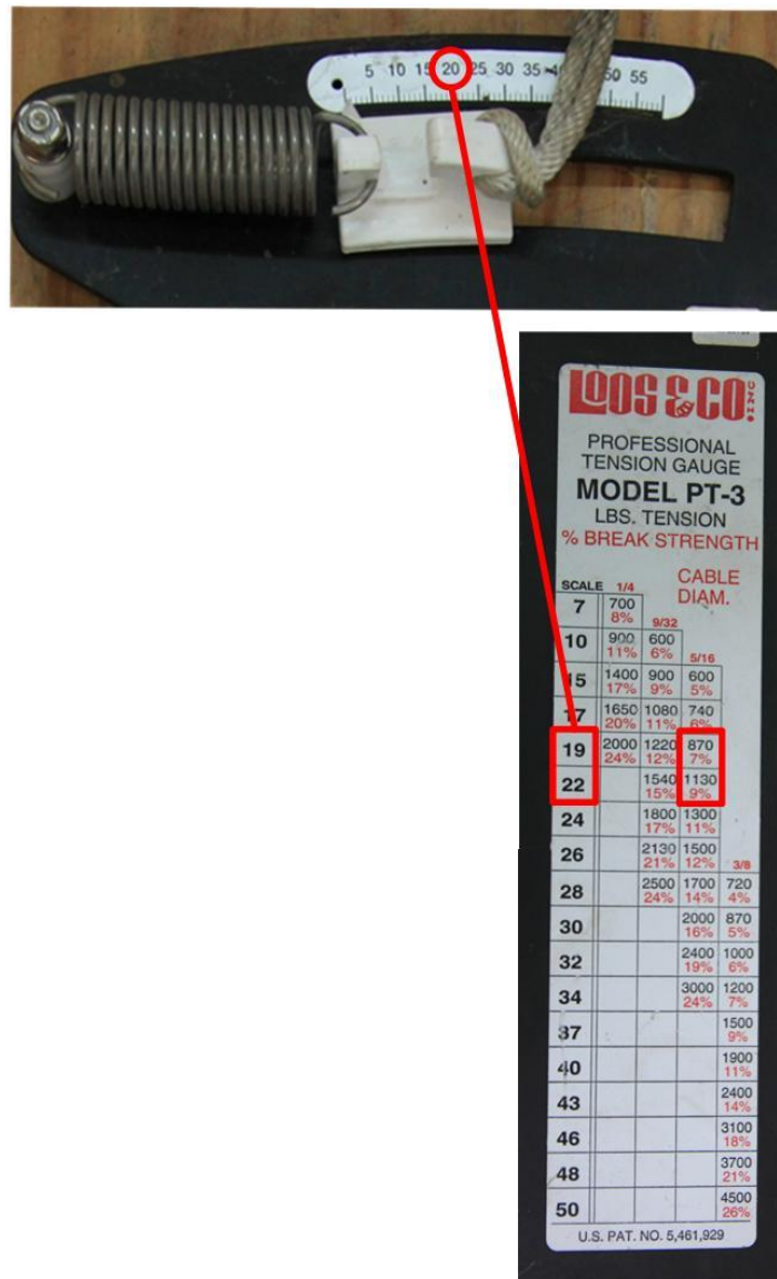
Picture 3-81: Tension Gauge
