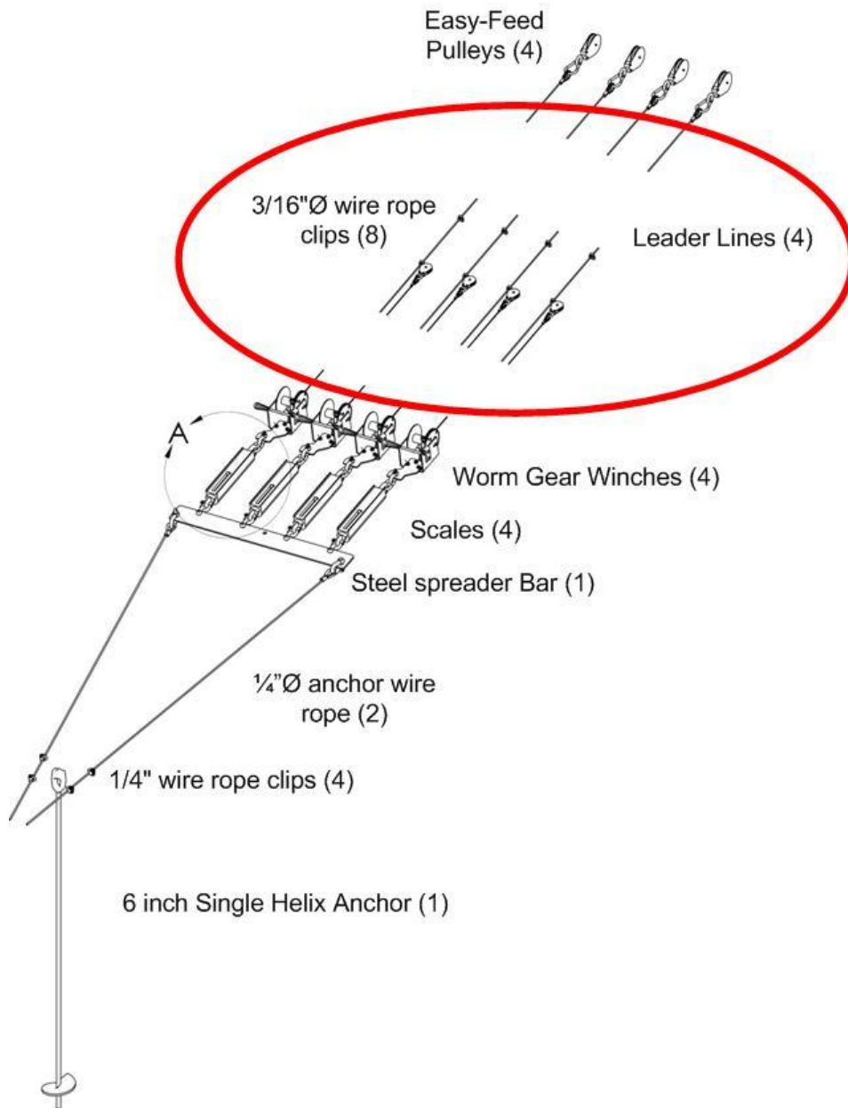
Picture E-7: Connecting the worm gear winch cables to the leader lines (Picture shows 80m tower set-up using 4 worm gears on each side. Super 60 utilizes 3 worm gears on each side).
