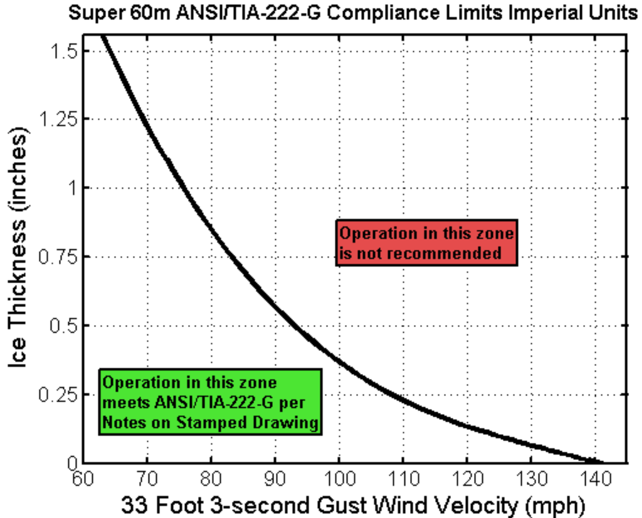
Picture A-4: Super 60m ANSI/TIA-222-G Compliance Limits Imperial Units
