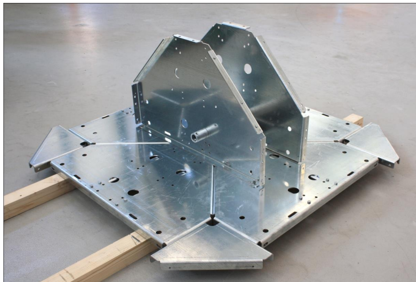
Picture 3-5: Baseplate Assembly
