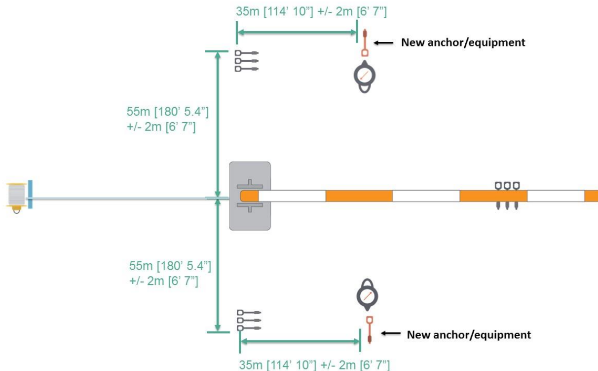
Picture 2-4: Layout drawing showing location of back stay tensioning system
