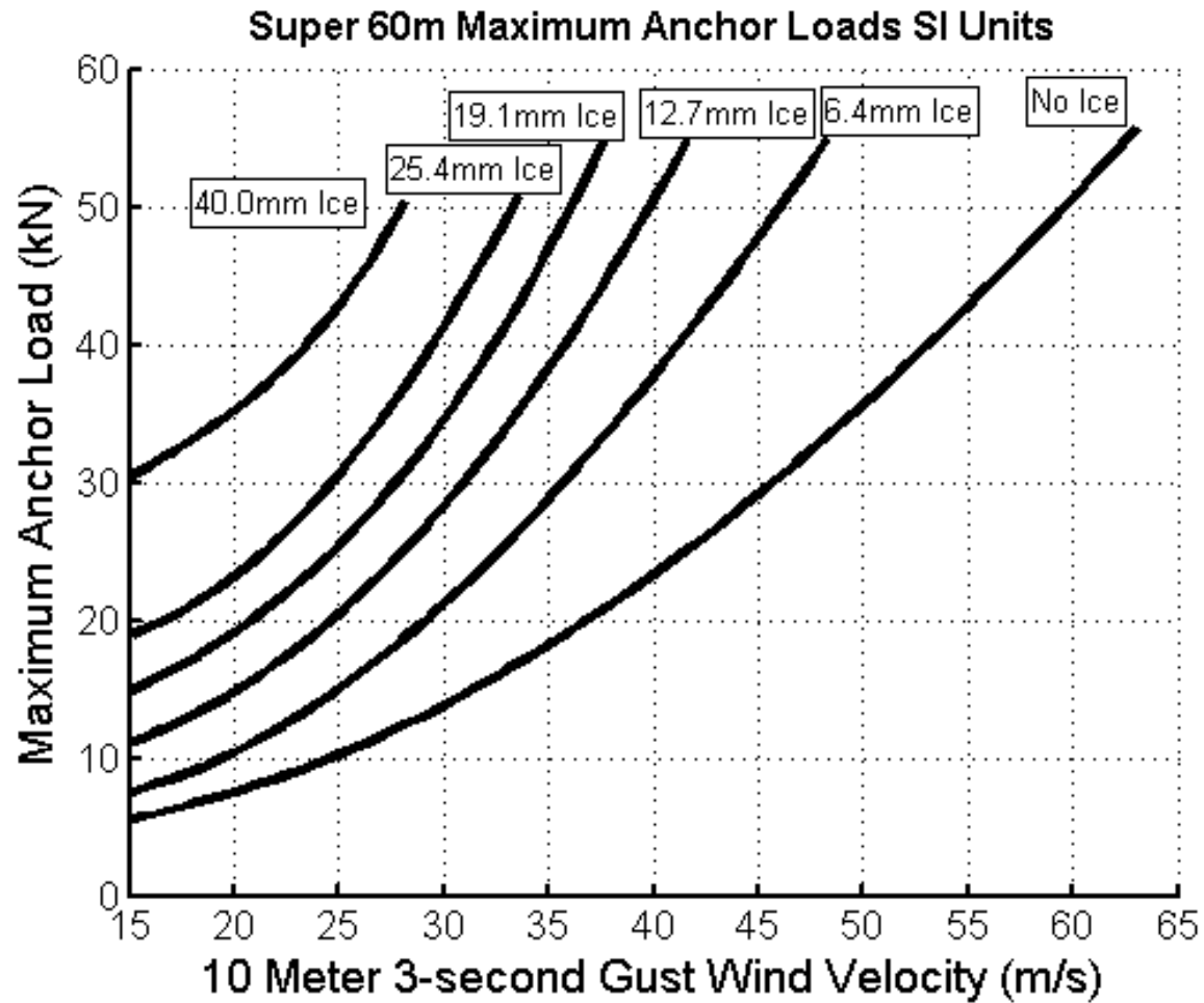
Picture A-7: Super 60 m XHD Maximum Anchor Loads SI Units
