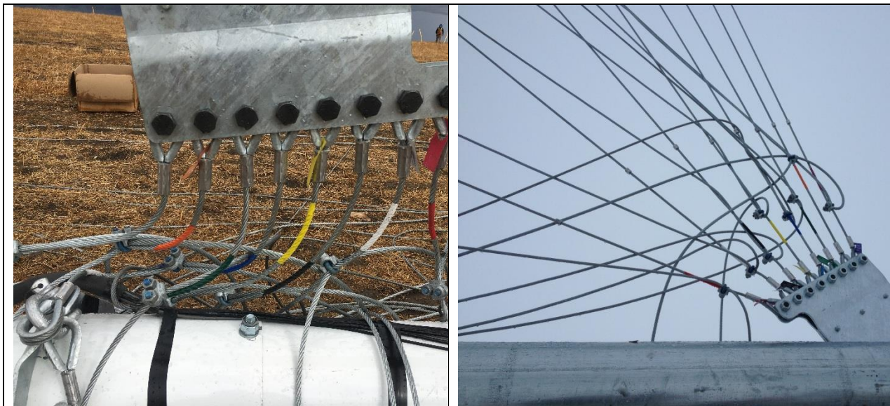
Picture 3-58: View of front guy wires attached to lifters (80 m tower) before and after tower raising
