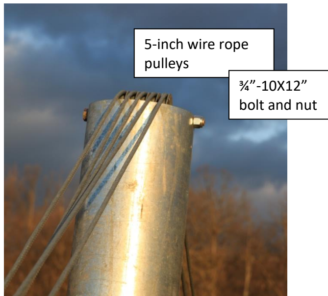
Picture 3-60: Helper ginpole pulleys with winch cable fully reeved
