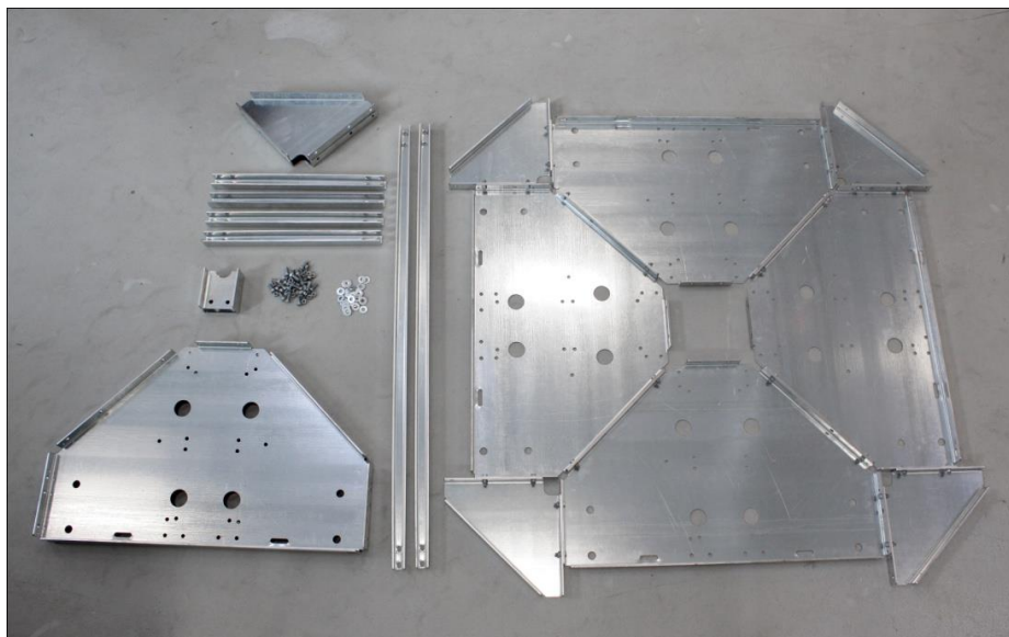
Picture 3-1: Baseplate Parts
