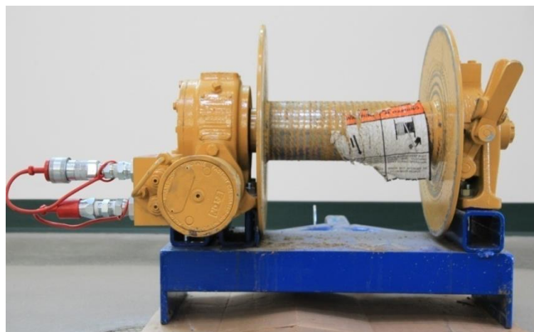
Picture 3-65: Super 60 Meter Bloom winch with mounting plate
