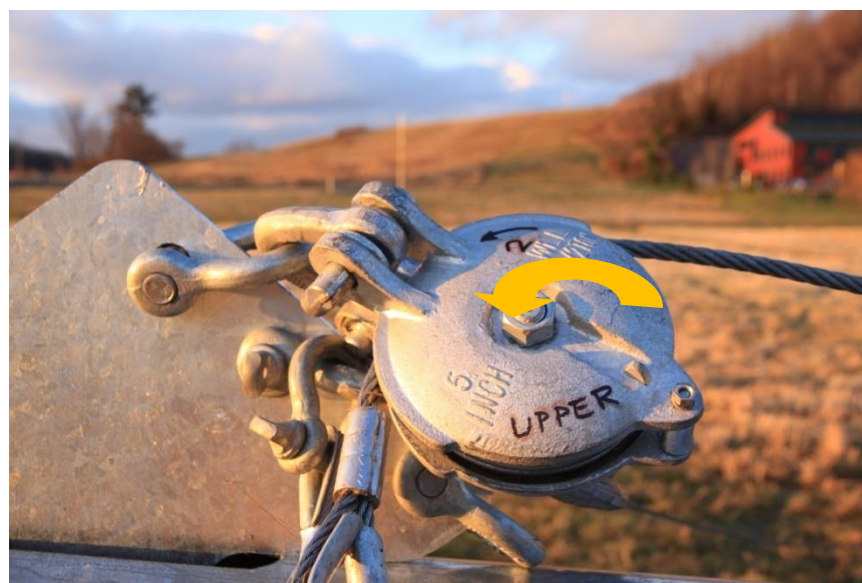
Picture 3-73: Reeving through pulley #2
