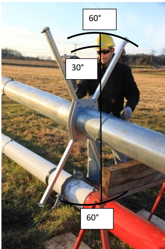
Picture 3-45: Install jumper struts
