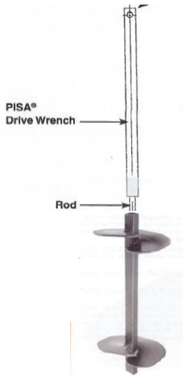
Picture B-3 Drive Wrench and Anchor Rod
