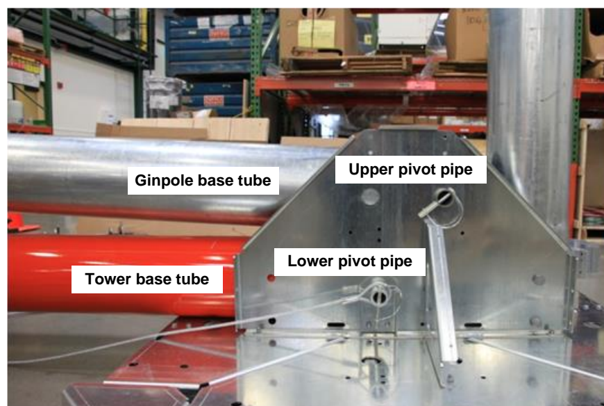
Picture 3-63: Complete baseplate and tower assembly ready for raising
