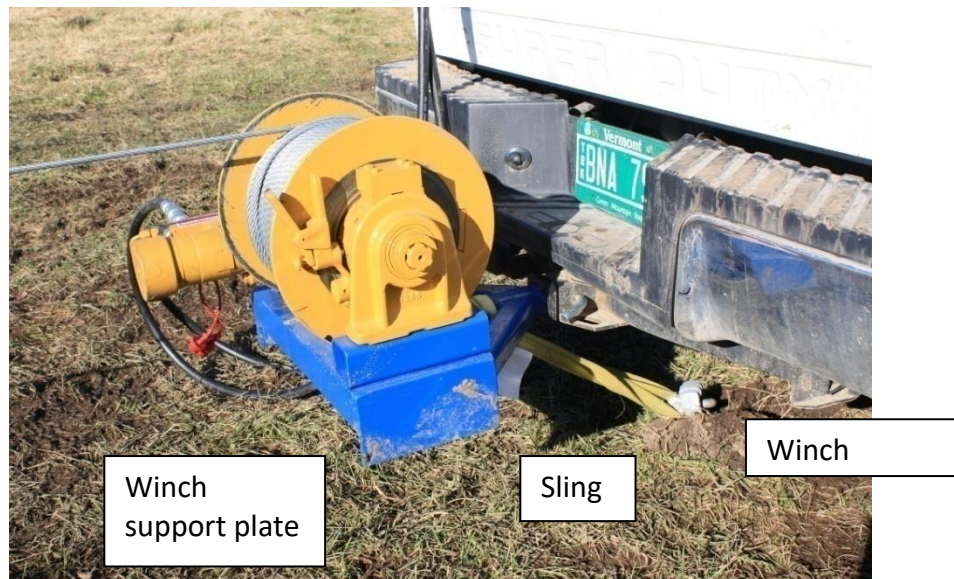
Picture 3-69: Correct winch assembly attached to winch anchor
