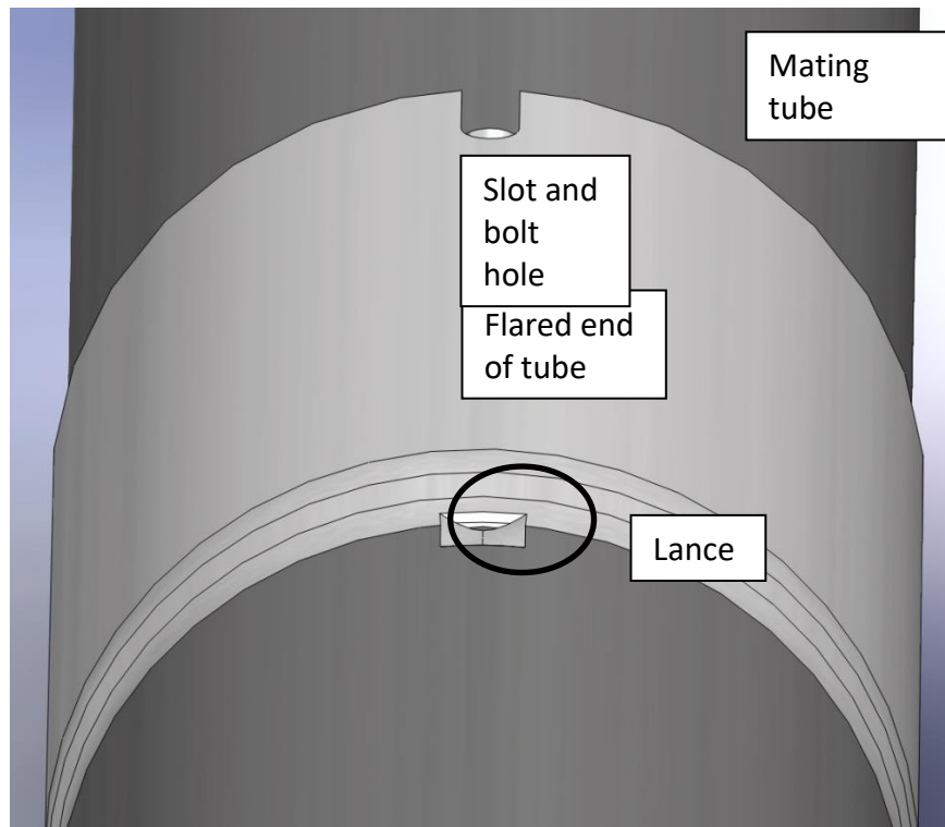
Picture 3-22: Tube lance and slot
