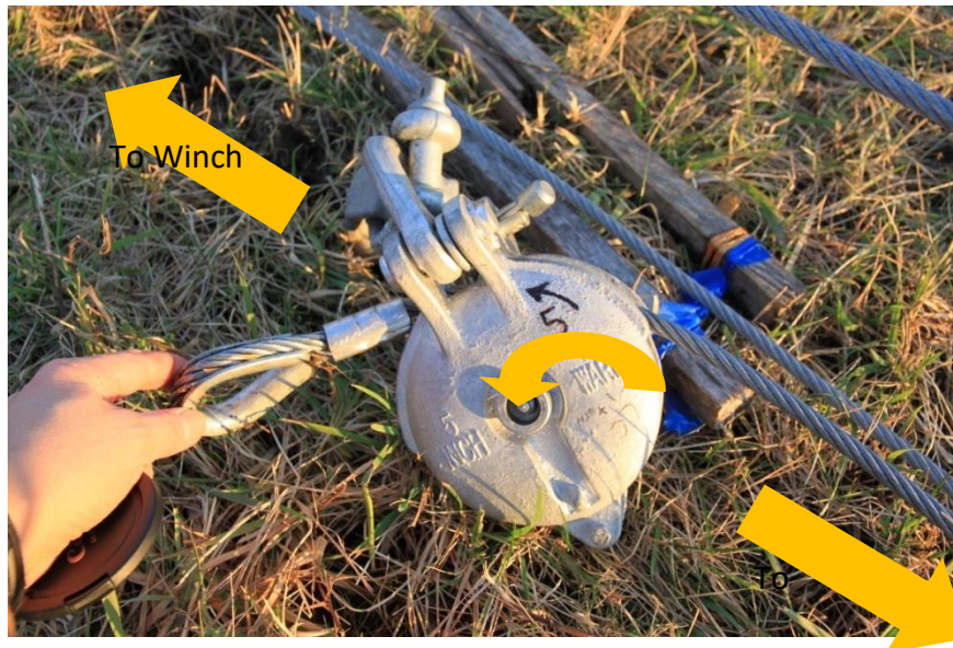
Picture 3-77: Reeving through pulley #5
