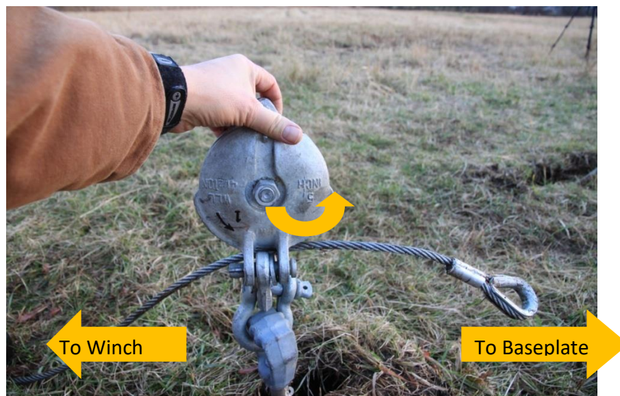
Picture 3-72: Reeving through pulley #1
