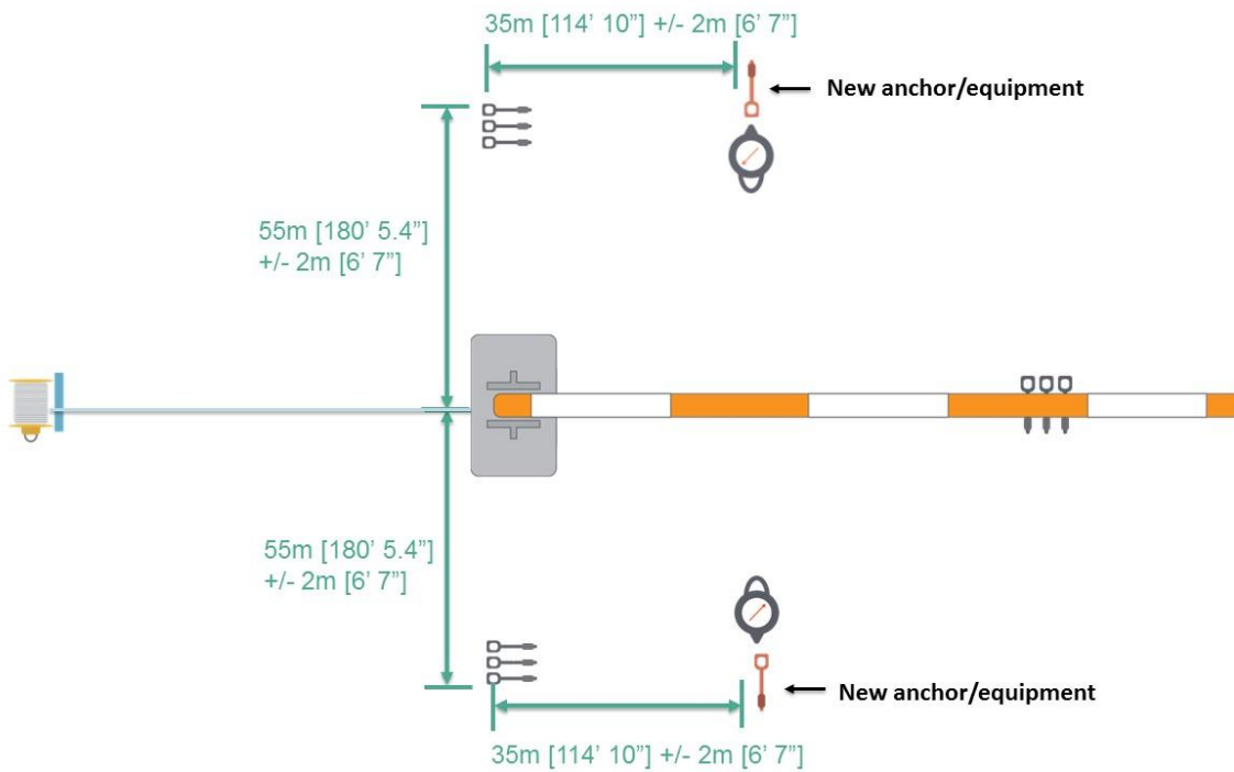
Picture E-3: Layout drawing showing placement of Back Guywire Tensioners/anchors
