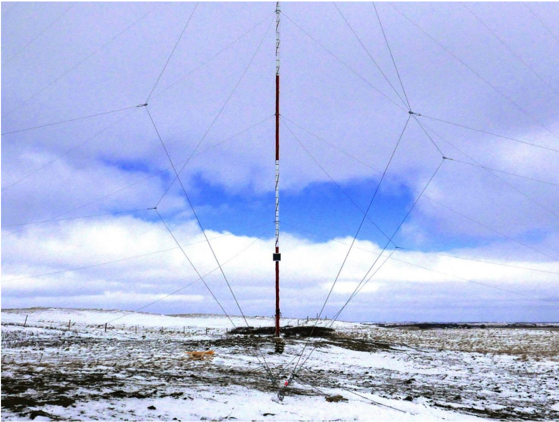
Picture E-11: View along tower showing acceptable back guywire/leader line tensions
